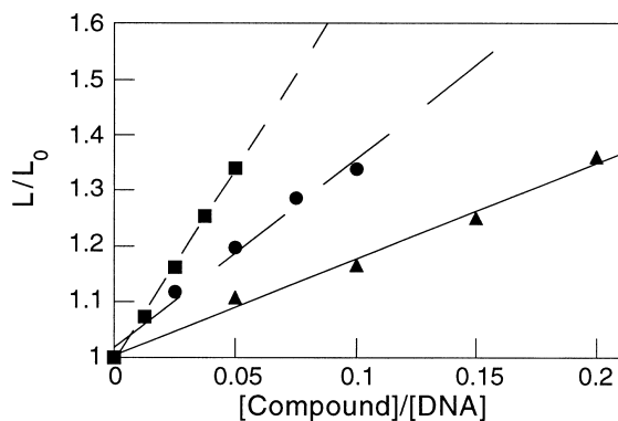
Figure 4. Viscometric data of dimer (▲, m=1.7 ), tetramer (●, m=3.4 ), and octamer (■, m=6.9 ) with sonicated calf thymus (CT) DNA in TE buffer (10 nM Tris, 50 mM NaCl, 1 mM EDTA).
