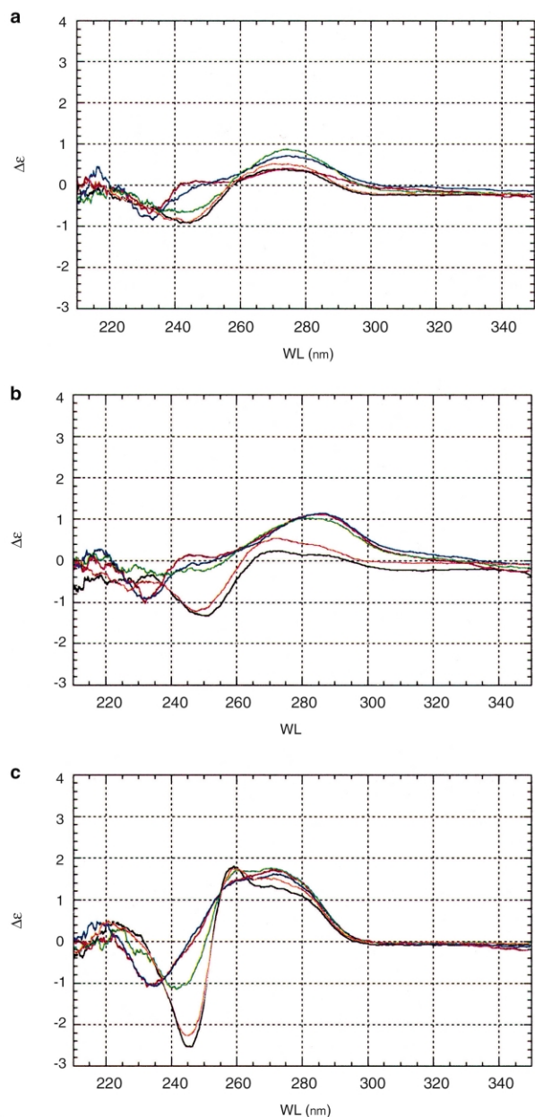
Figure 6. Circular dichroism traces of intercalators with DNA; a, calf thymus DNA; b, poly(dGdC) 2 ; c, poly(A):poly(dT); black, DNA alone; red, DNA and dimer; blue, DNA and octamer; green, DNA and monomer; orange, DNA and ethidium bromide.
